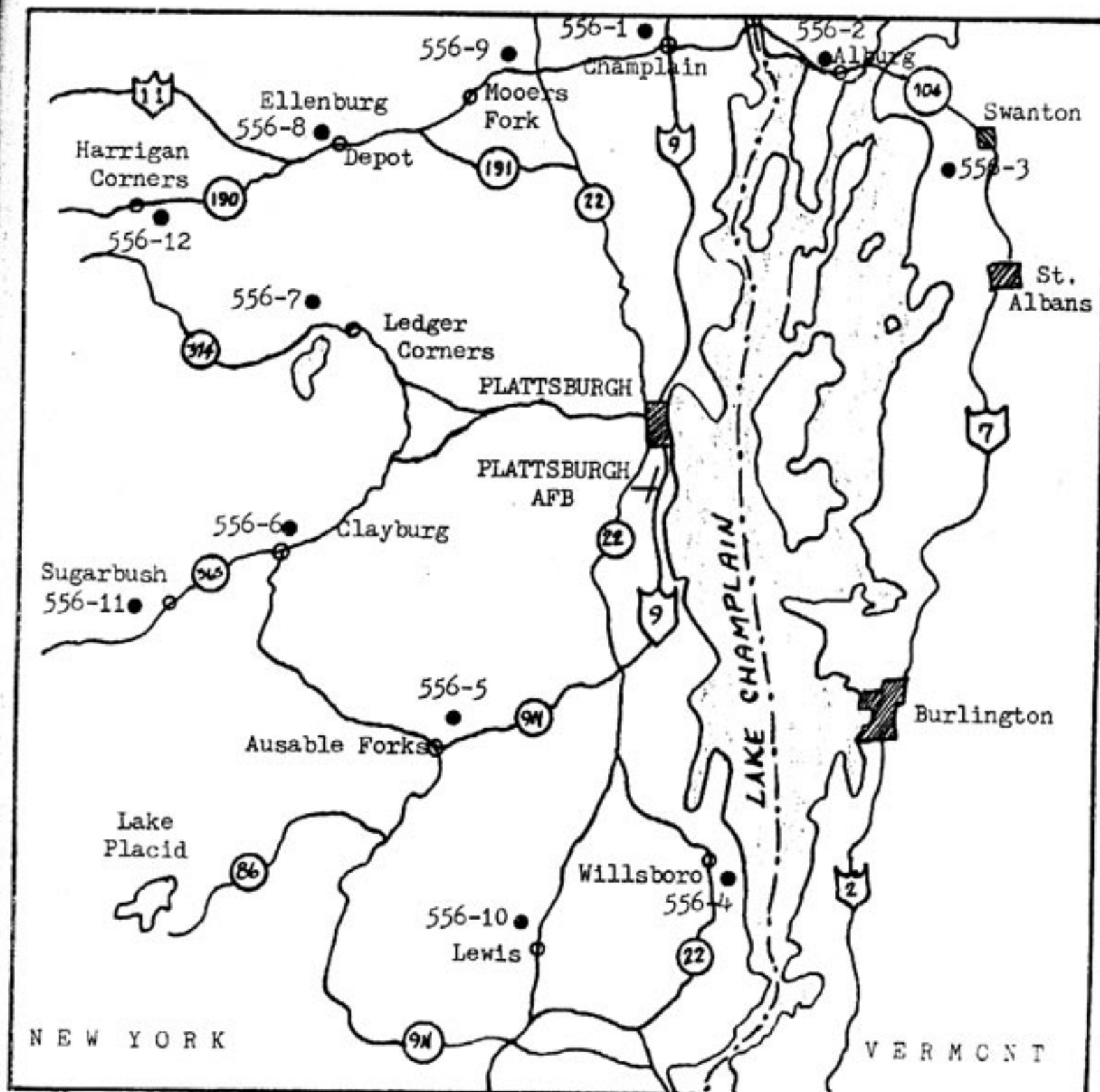
Figure 28. Plattsburgh AFB: ATLAS F Sites
