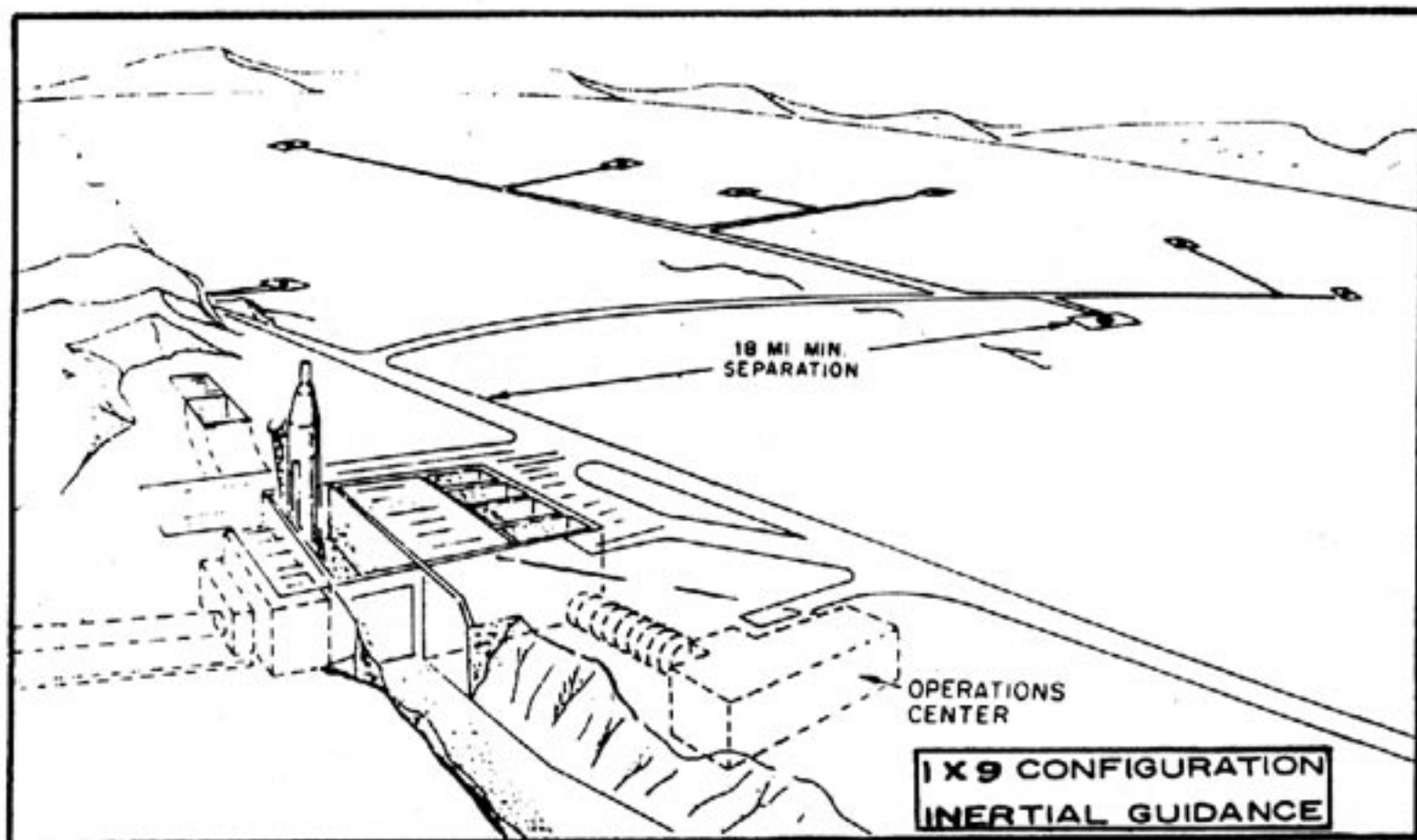
Figure 4. ATLAS E: Typical Complex Layout
