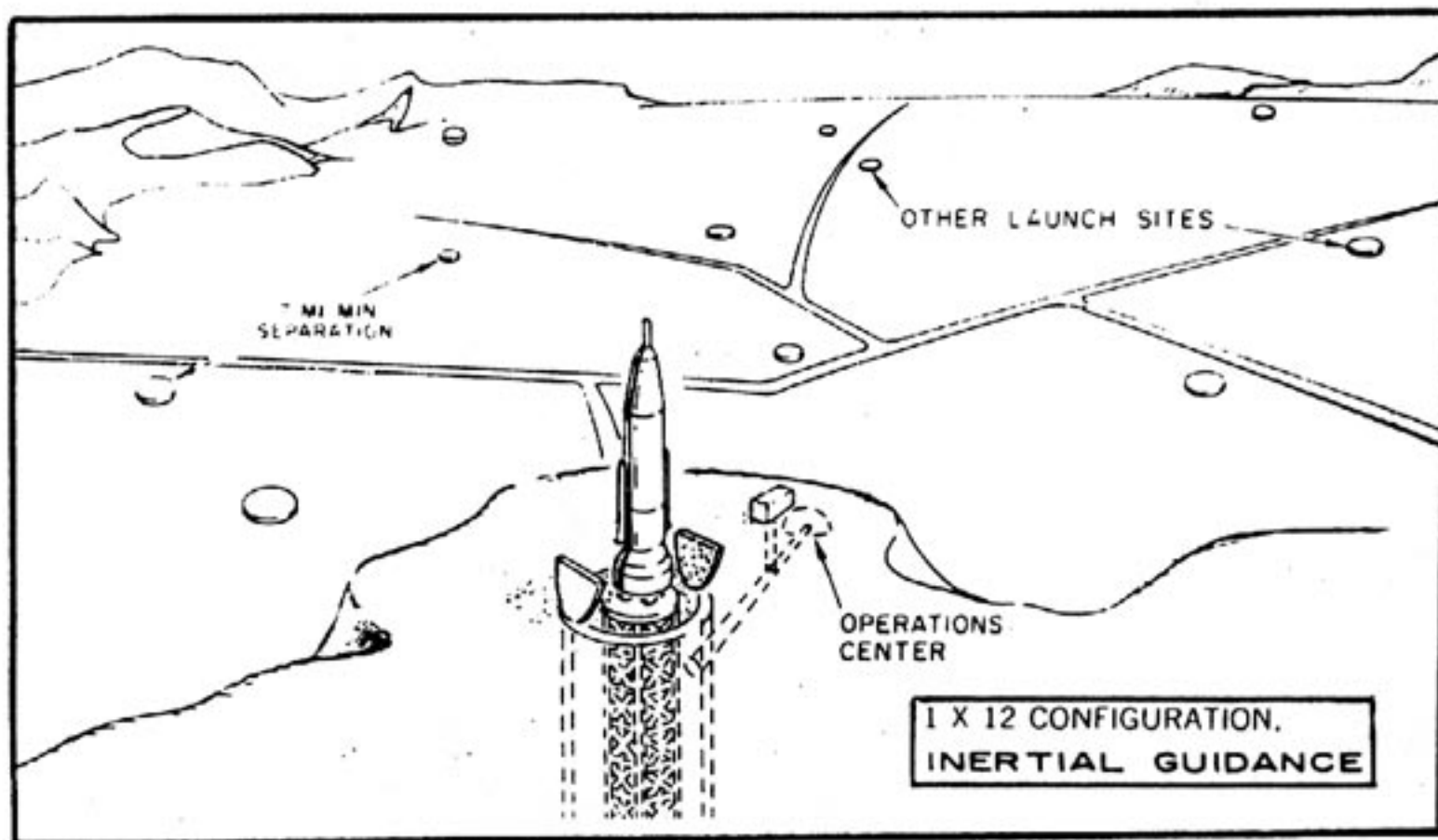
Figure 5. ATLAS F: Typical Complex Layout
