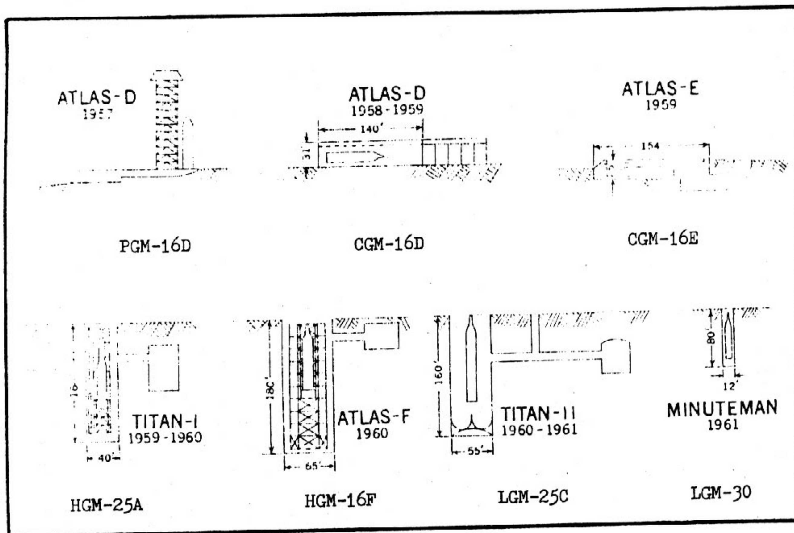
Figure 2. Evolution of ICBM Launchers
