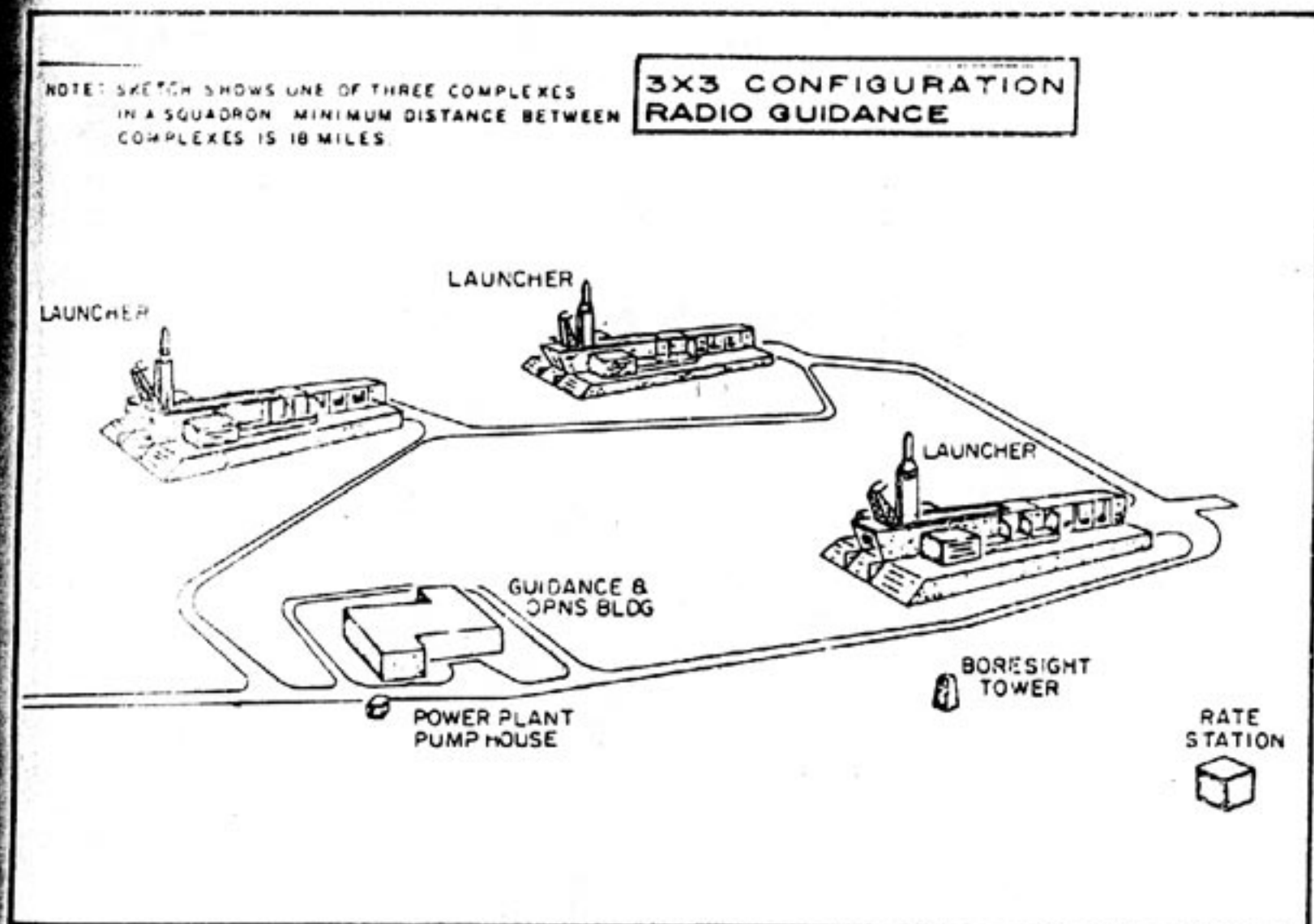
Figure 3. ATLAS D: Typical Complex Layout
